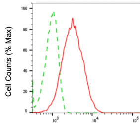
BCL10 Immune Signaling Adaptor-Alexa Fluor® 647
