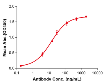
ELISA plate pre-coated Antigen protein, can bind Denosumab biosimilar in a linear range of 3.91-125 ng/mL.
