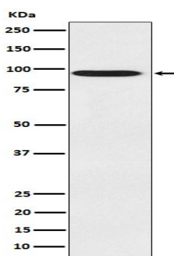
Western blot analysis of CDT2 in 293T lysates using CDT2 antibody.
