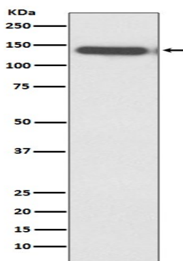
Western blot analysis of Ctip2 in Jurkat lysates using Ctip2 antibody.
